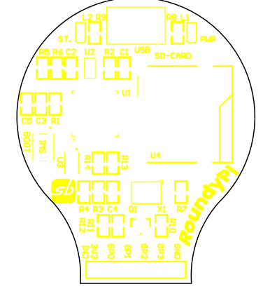
Top Overlay (Scale 1.2361:1)
