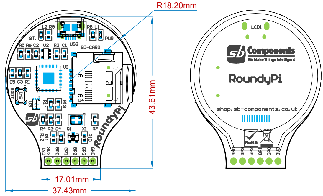
Top Overlay (Scale 1.2361:1)
