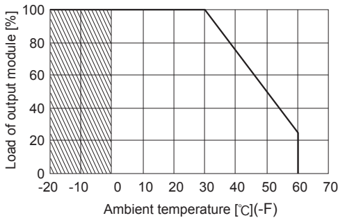
Fig. 6.2 Derating curve characteristics resulting from ambient temperature (-F)
