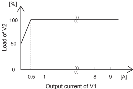
Fig. 5.2 Minimum output current of V1
