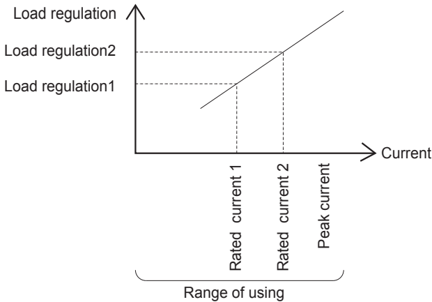
Fig. 5.1 The relationship between rated current and load regulation
