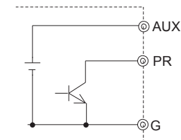
Fig. 3.4 PR internal circuit
