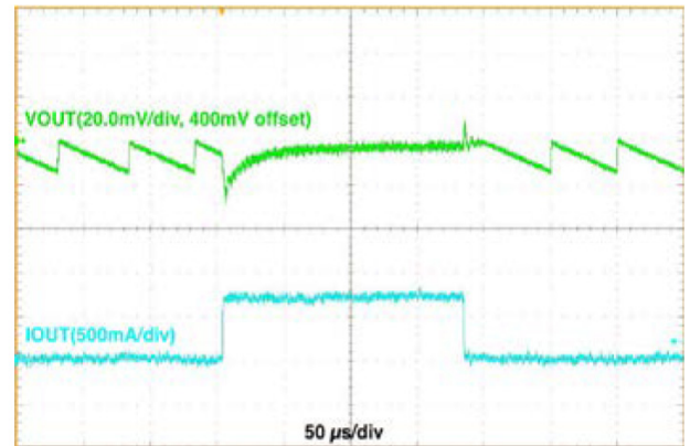
Figure 14. Load Transient, V_{IN} = 3.6\text{ V} , V_{OUT} = 0.4\text{ V} , 10 mA \Leftrightarrow 770 mA, 200 ns Edge, Auto Mode
