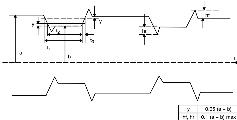
Figure 3. 10% Modulation Waveform
