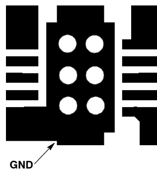
Figure 21. Recommended Footprint
