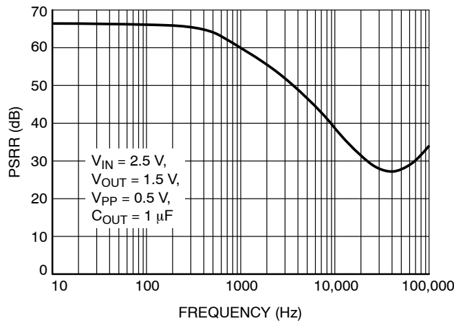
Figure 31. PSRR vs. Frequency (V out = 1.5 V)
