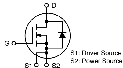
N-CHANNEL MOSFET
